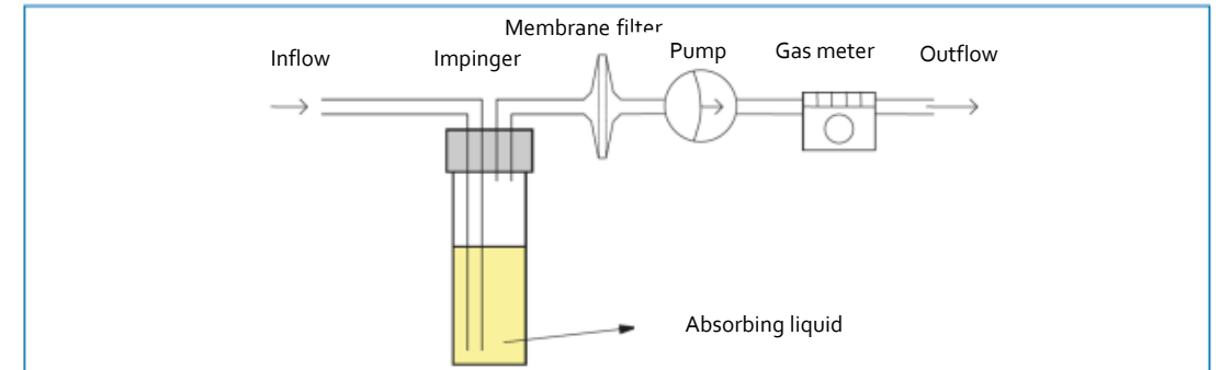
Diagram of the AGI-30 sampling system
