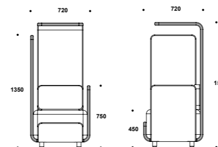
402HYL AREA CHAIR HYBRID LEFT
