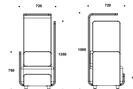
402HYR AREA CHAIR HYBRID RIGHT
