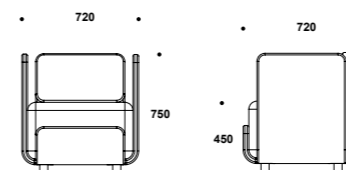
402CM AREA CHAIR MEDIUM
